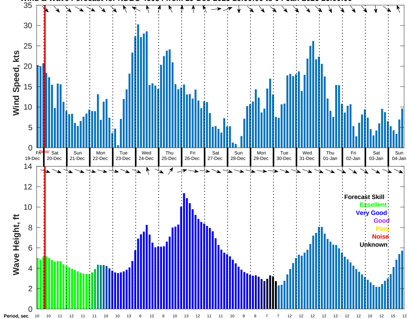
Wind & Wave Forecast for NDBC 46054 from 19-Dec-2025 16:00:00 to 04-Jan-2026 16:00:00
