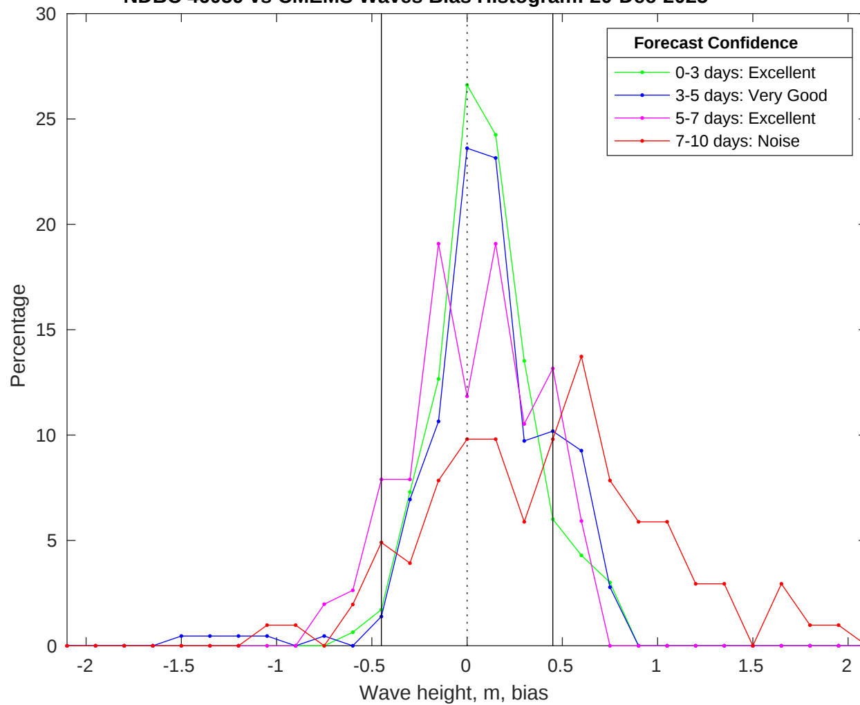
NDBC 46059 vs CMEMS Waves Bias Histogram: 20-Dec-2025
