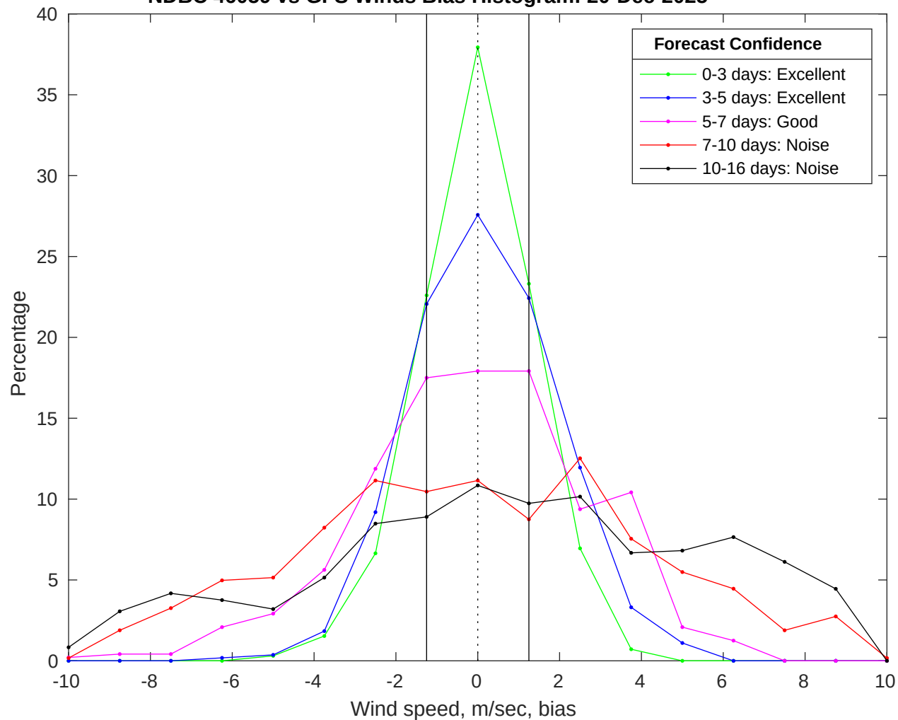
NDBC 46059 vs GFS Winds Bias Histogram: 20-Dec-2025
