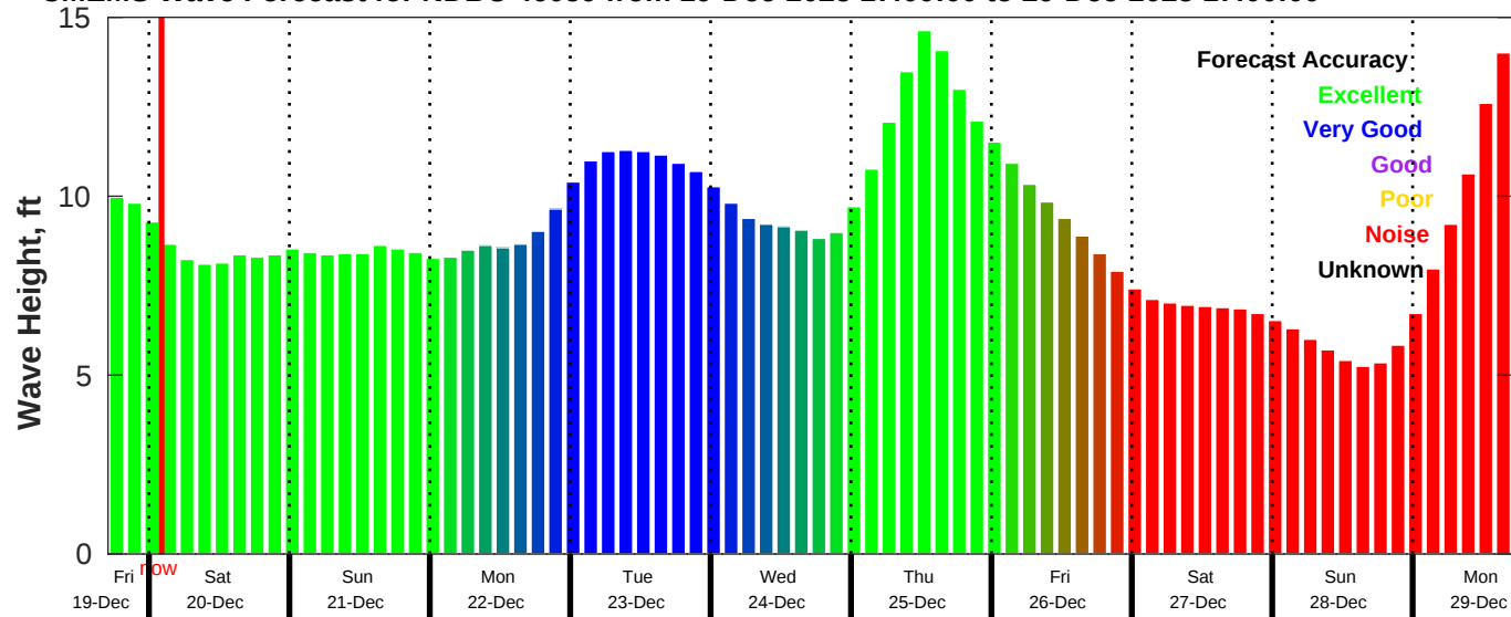
CMEMS Wave Forecast for NDBC 46059 from 19-Dec-2025 17:00:00 to 29-Dec-2025 17:00:00
