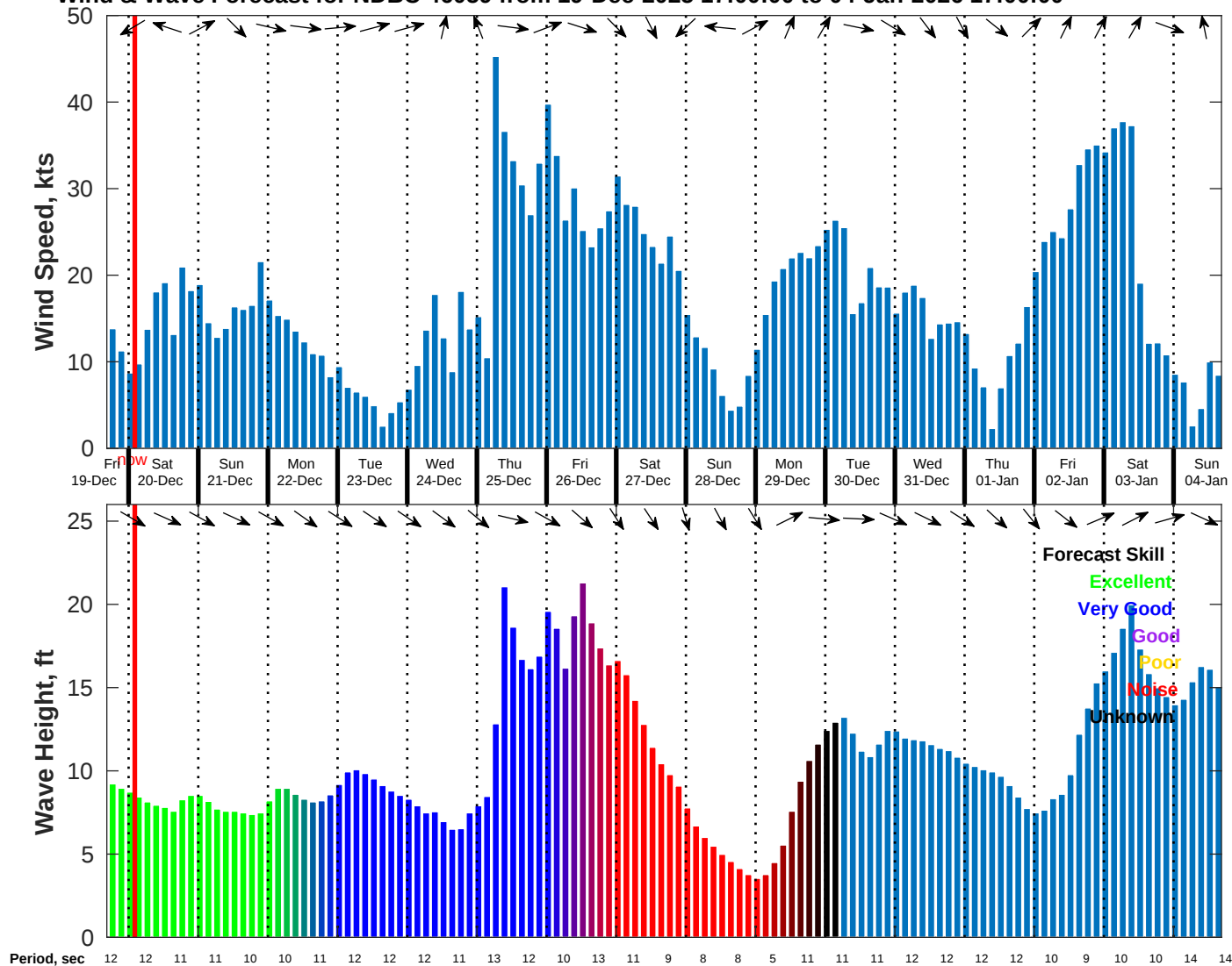
Wind & Wave Forecast for NDBC 46059 from 19-Dec-2025 17:00:00 to 04-Jan-2026 17:00:00
