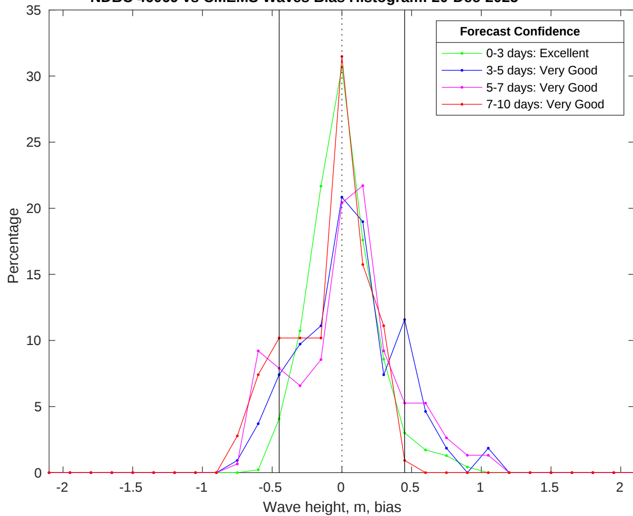
NDBC 46069 vs CMEMS Waves Bias Histogram: 20-Dec-2025
