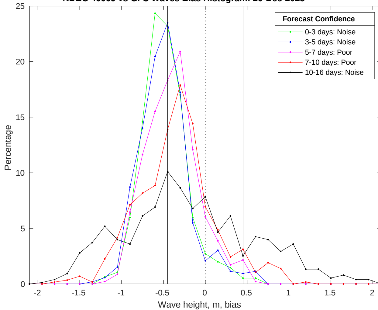
NDBC 46069 vs GFS Waves Bias Histogram: 20-Dec-2025
