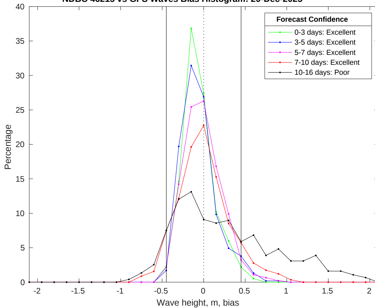
NDBC 46215 vs GFS Waves Bias Histogram: 20-Dec-2025
