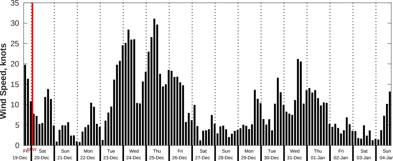
GFS Wind Speed Forecast for NDBC 46215 from 19-Dec-2025 16:00:00 to 04-Jan-2026 16:00:00
