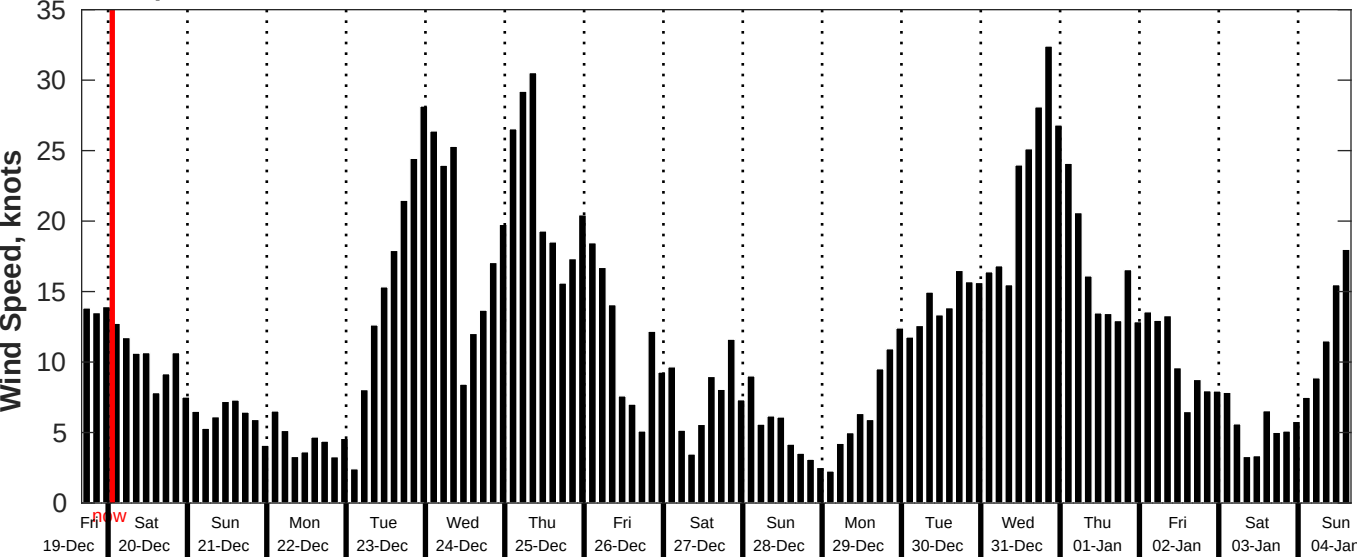
GFS Wind Speed Forecast for NDBC 46259 from 19-Dec-2025 16:00:00 to 04-Jan-2026 16:00:00
