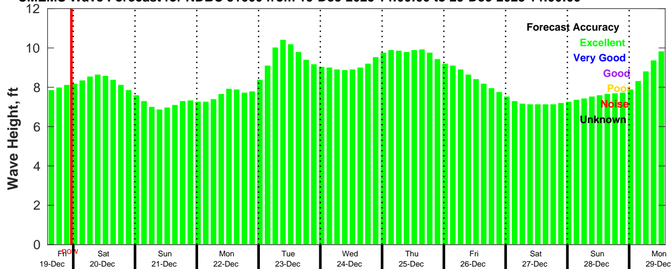
CMEMS Wave Forecast for NDBC 51000 from 19-Dec-2025 14:00:00 to 29-Dec-2025 14:00:00
