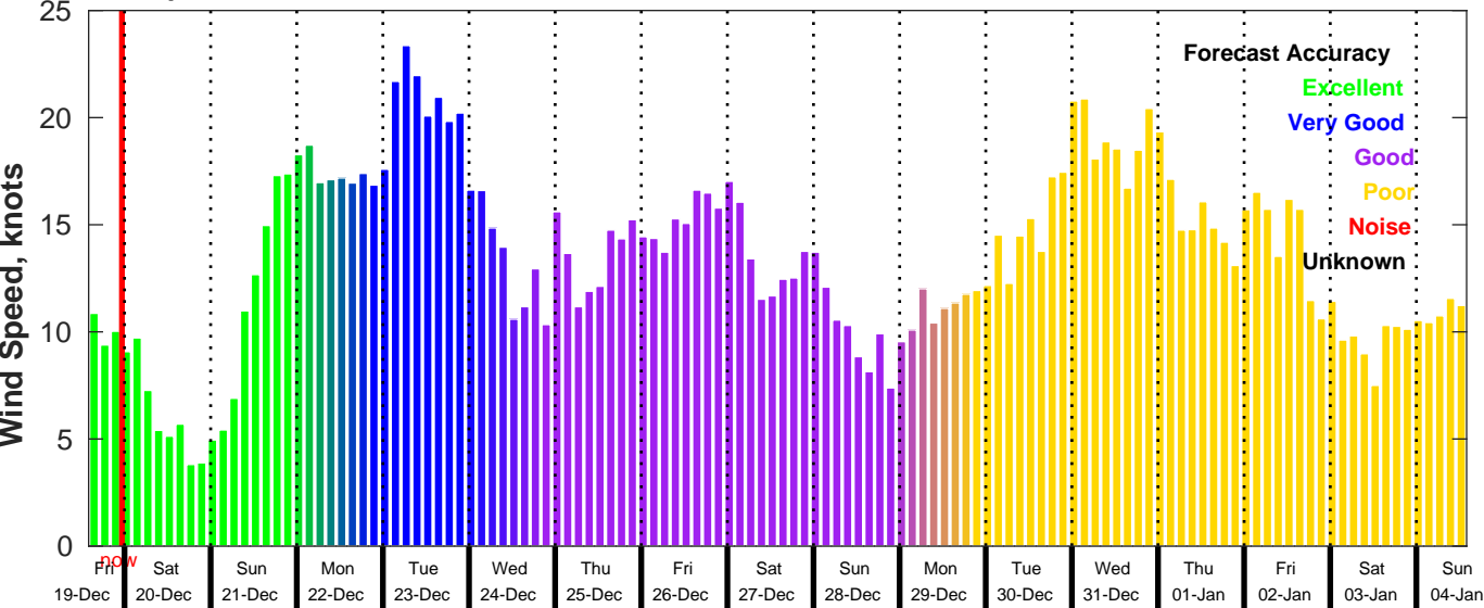
GFS Wind Speed Forecast for NDBC 51000 from 19-Dec-2025 14:00:00 to 04-Jan-2026 14:00:00
