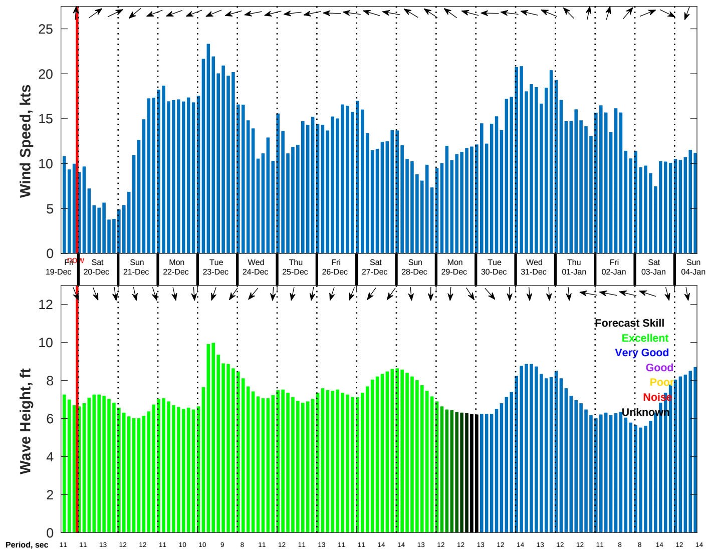
Wind & Wave Forecast for NDBC 51000 from 19-Dec-2025 14:00:00 to 04-Jan-2026 14:00:00
