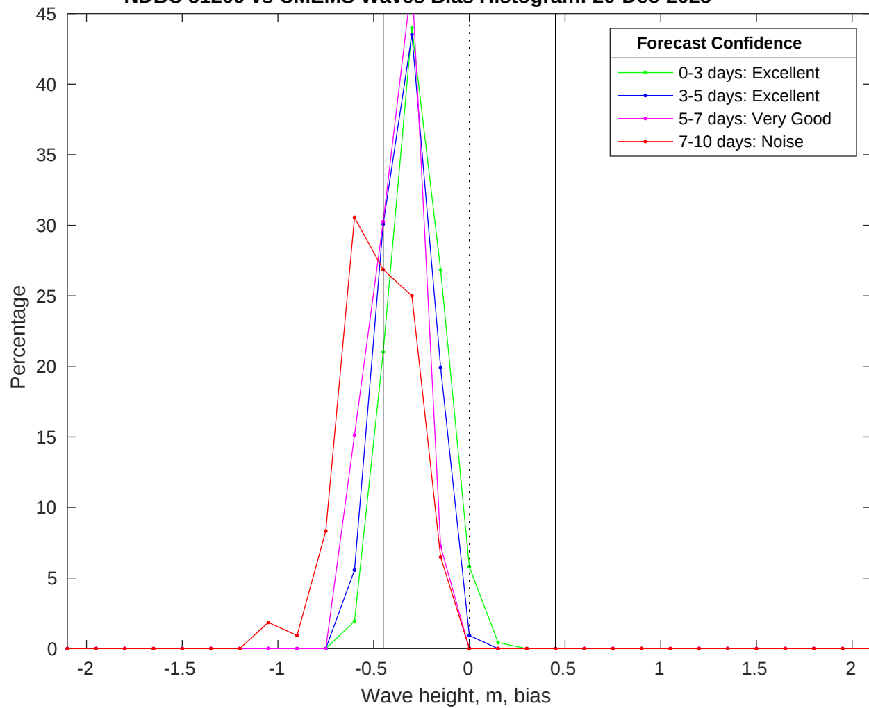
NDBC 51209 vs CMEMS Waves Bias Histogram: 20-Dec-2025
