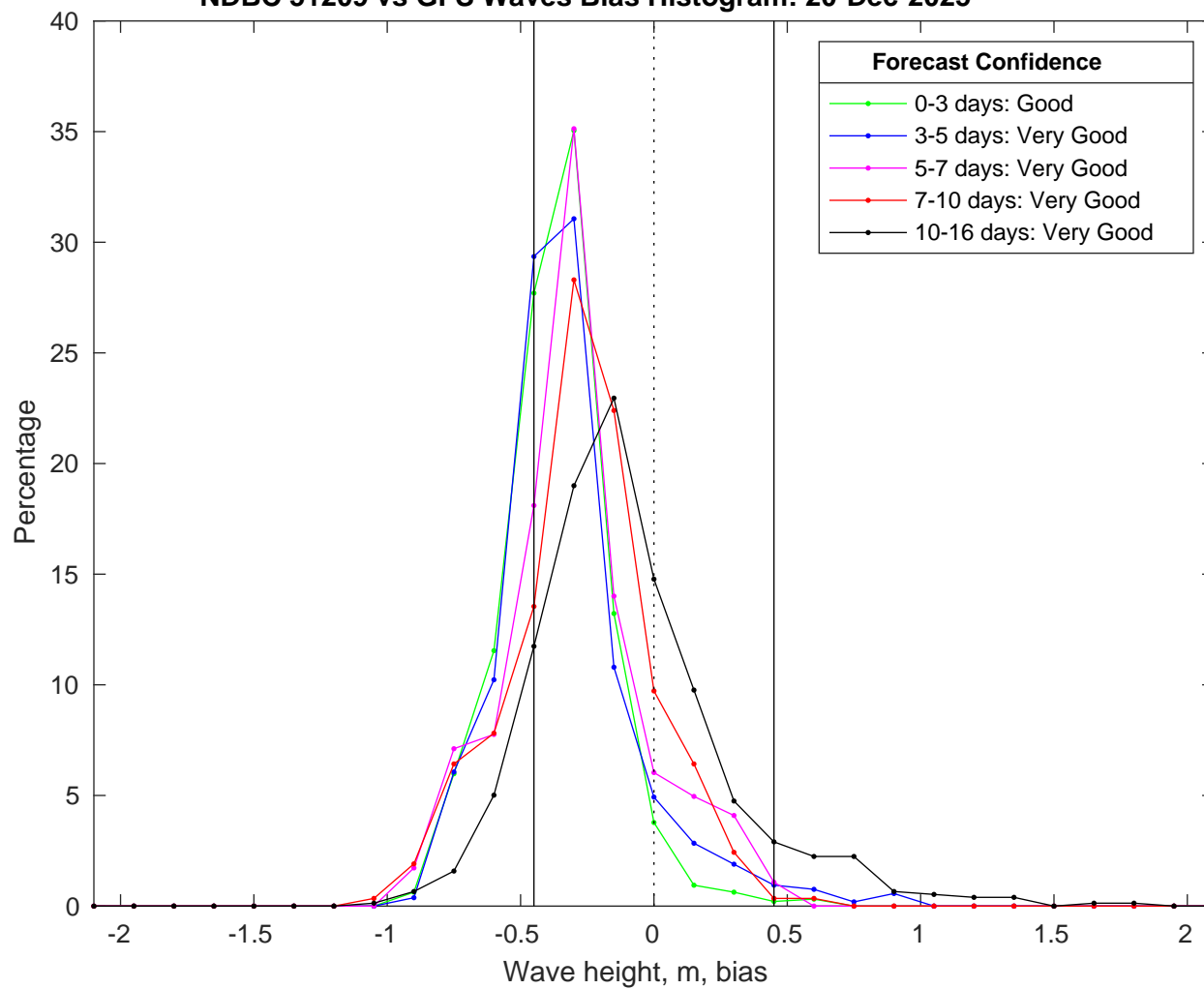
NDBC 51209 vs GFS Waves Bias Histogram: 20-Dec-2025
