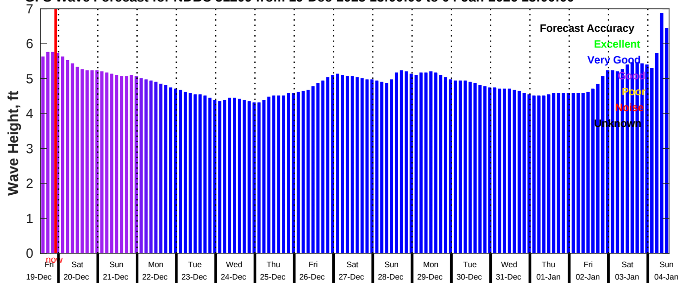
GFS Wave Forecast for NDBC 51209 from 19-Dec-2025 13:00:00 to 04-Jan-2026 13:00:00
