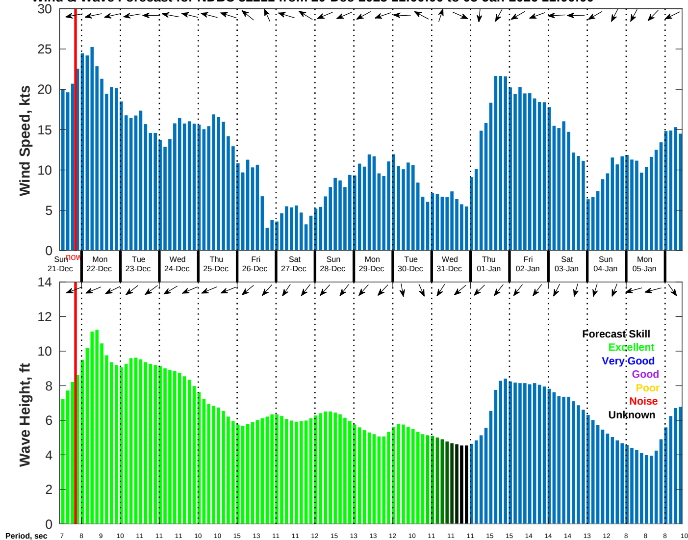
Wind & Wave Forecast for NDBC 52211 from 20-Dec-2025 11:00:00 to 05-Jan-2026 11:00:00
