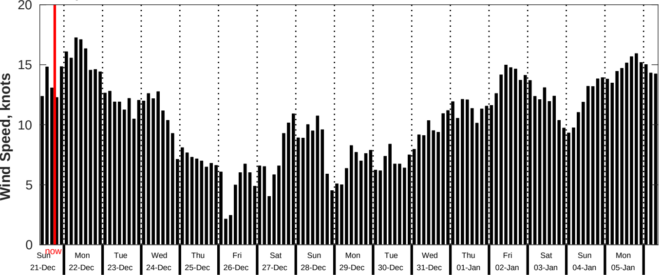
GFS Wind Speed Forecast for NDBC 52212 from 20-Dec-2025 09:00:00 to 05-Jan-2026 09:00:00
