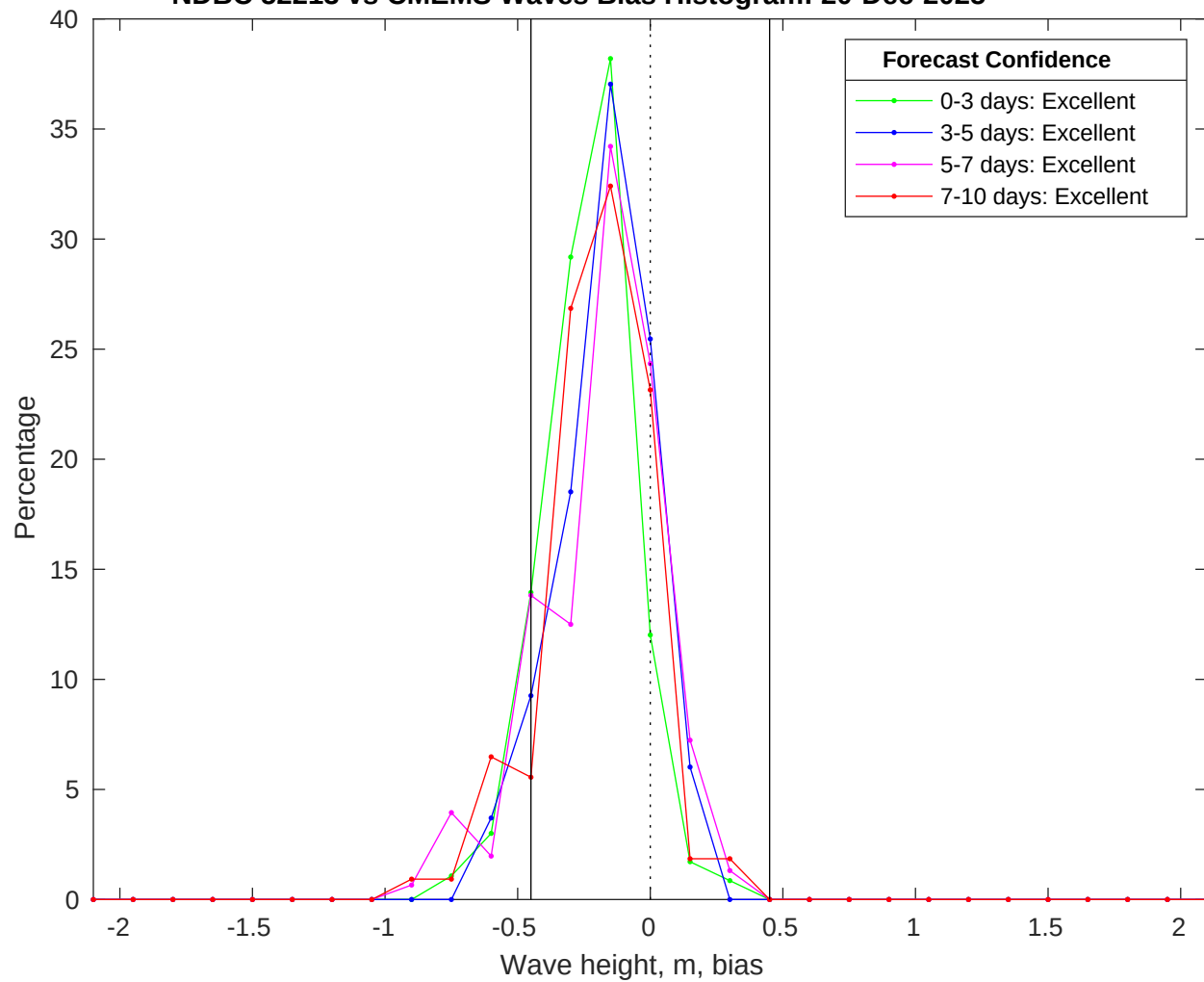
NDBC 52213 vs CMEMS Waves Bias Histogram: 20-Dec-2025
