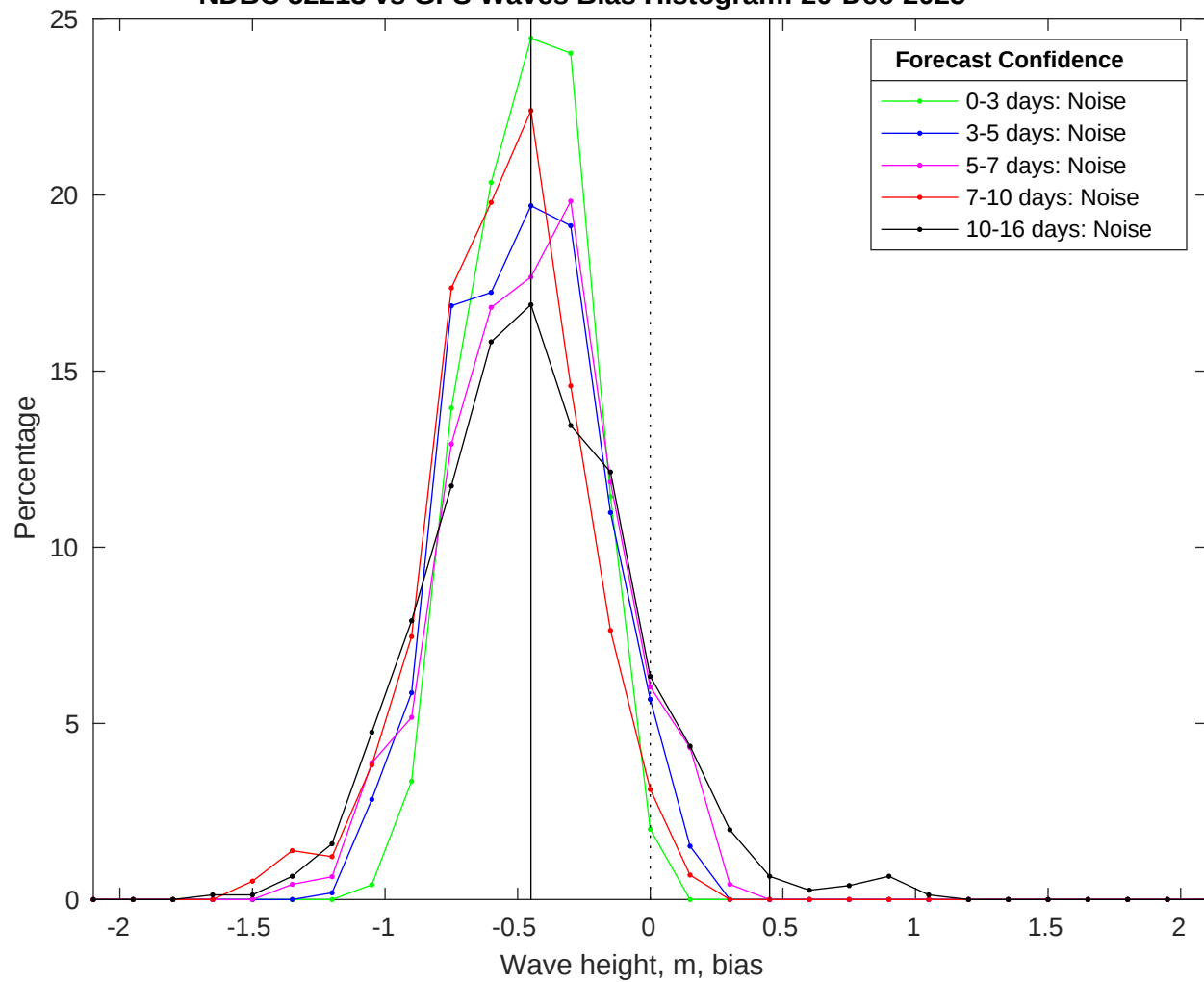
NDBC 52213 vs GFS Waves Bias Histogram: 20-Dec-2025
