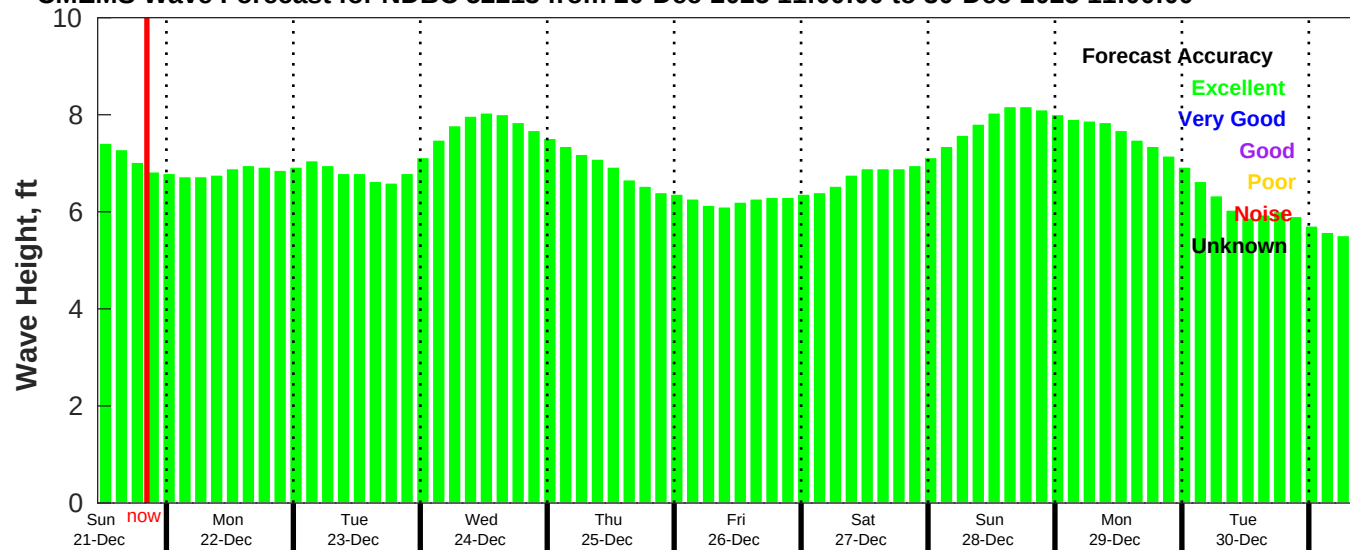
CMEMS Wave Forecast for NDBC 52213 from 20-Dec-2025 11:00:00 to 30-Dec-2025 11:00:00
