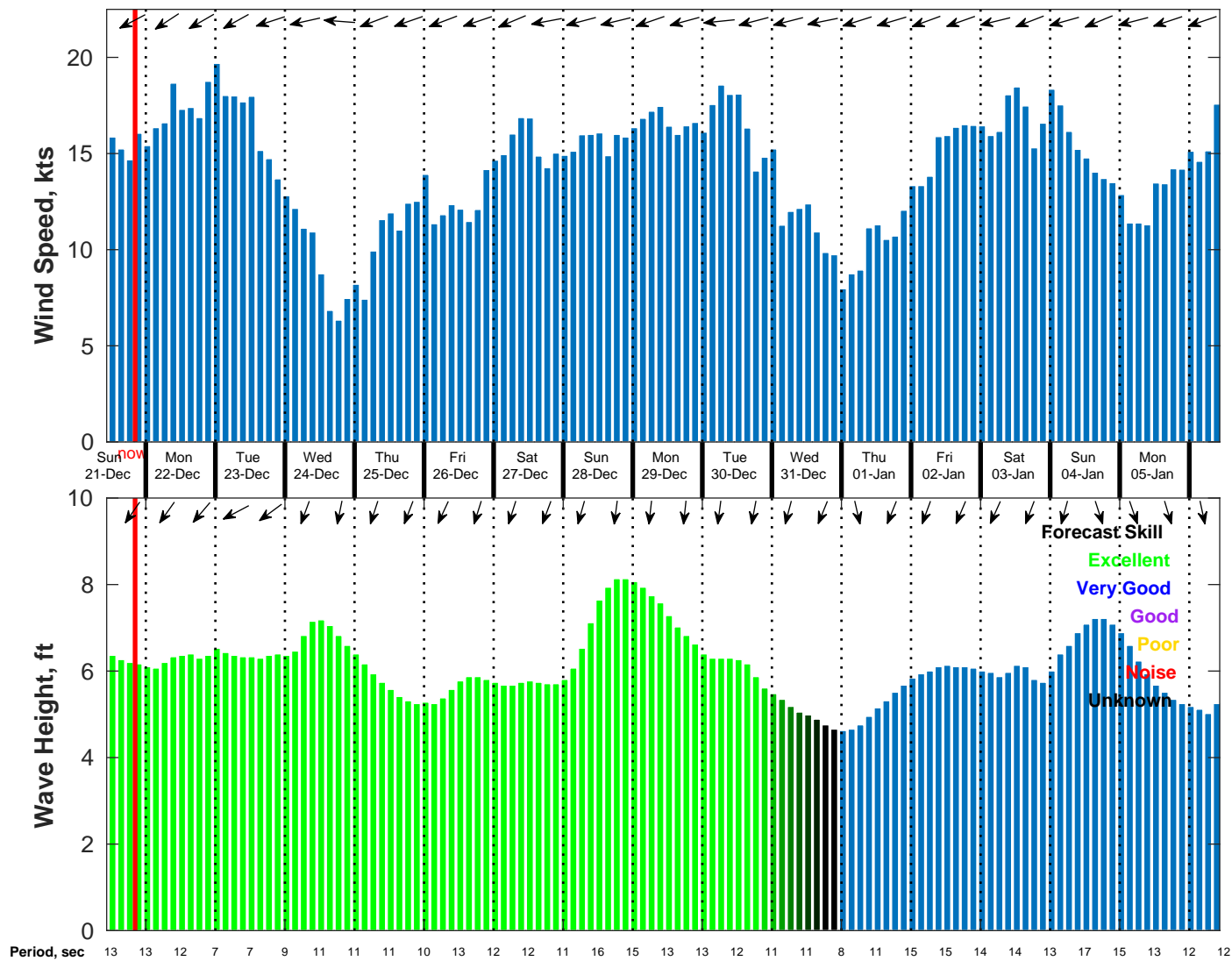
Wind & Wave Forecast for NDBC 52213 from 20-Dec-2025 11:00:00 to 05-Jan-2026 11:00:00
