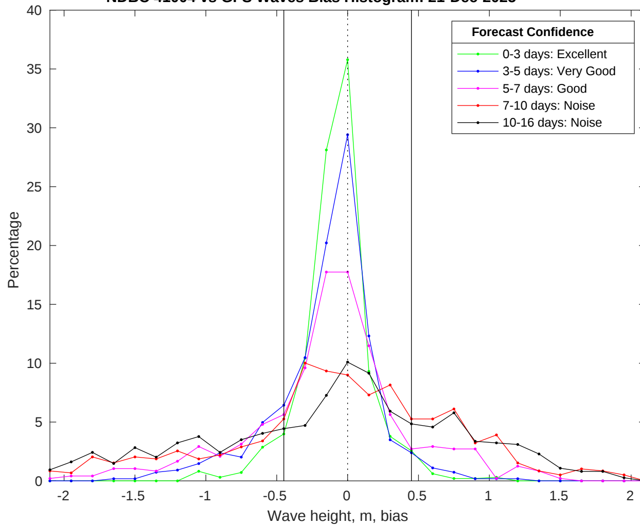
NDBC 41004 vs GFS Waves Bias Histogram: 21-Dec-2025
