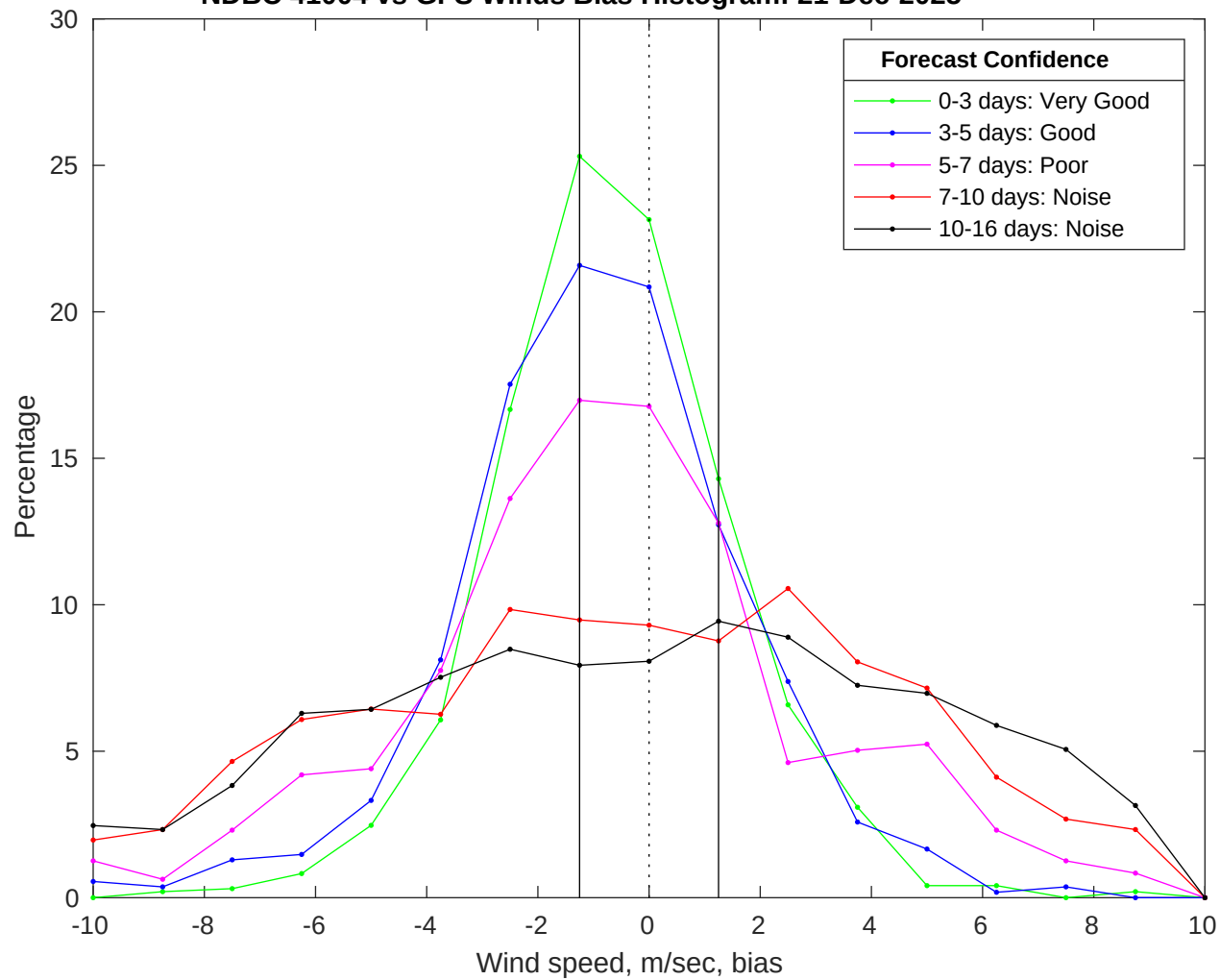
NDBC 41004 vs GFS Winds Bias Histogram: 21-Dec-2025
