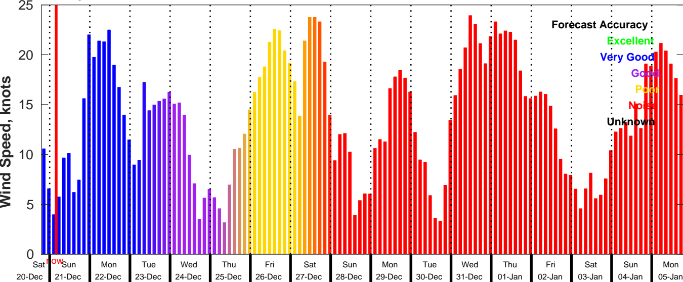
GFS Wind Speed Forecast for NDBC 41004 from 20-Dec-2025 19:00:00 to 05-Jan-2026 19:00:00
