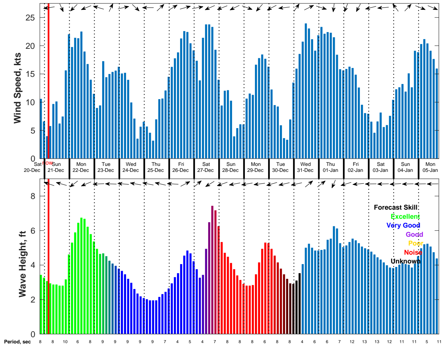
Wind & Wave Forecast for NDBC 41004 from 20-Dec-2025 19:00:00 to 05-Jan-2026 19:00:00
