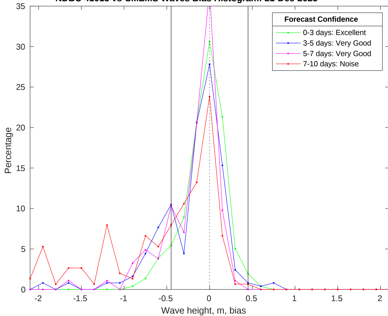
NDBC 41013 vs CMEMS Waves Bias Histogram: 21-Dec-2025
