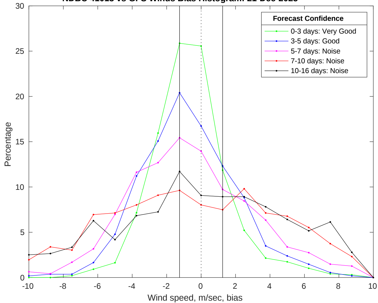
NDBC 41013 vs GFS Winds Bias Histogram: 21-Dec-2025
