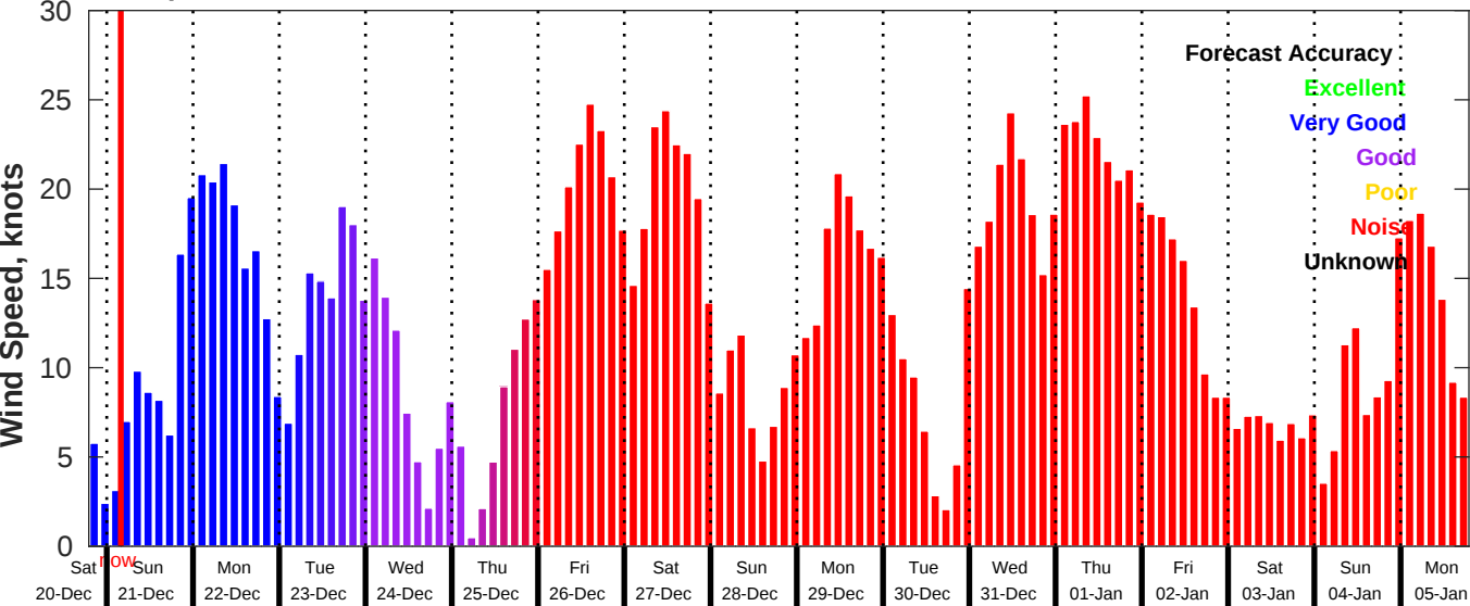
GFS Wind Speed Forecast for NDBC 41013 from 20-Dec-2025 19:00:00 to 05-Jan-2026 19:00:00
