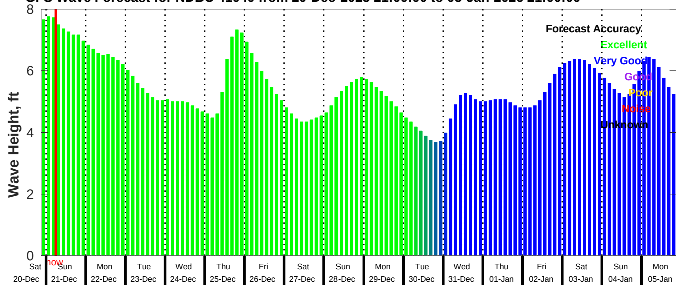
GFS Wave Forecast for NDBC 41040 from 20-Dec-2025 21:00:00 to 05-Jan-2026 21:00:00
