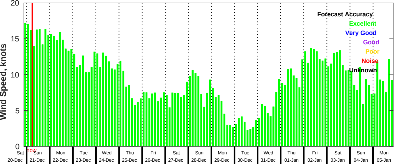
GFS Wind Speed Forecast for NDBC 41040 from 20-Dec-2025 21:00:00 to 05-Jan-2026 21:00:00
