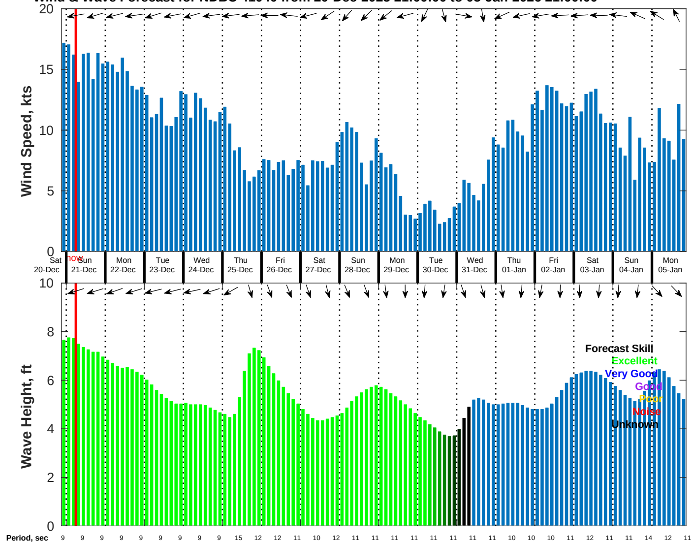
Wind & Wave Forecast for NDBC 41040 from 20-Dec-2025 21:00:00 to 05-Jan-2026 21:00:00
