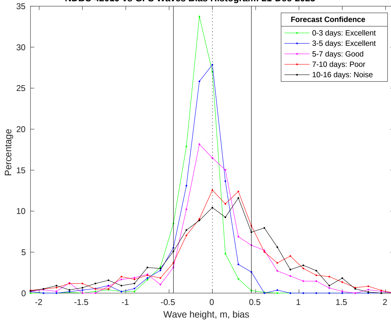
NDBC 42019 vs GFS Waves Bias Histogram: 21-Dec-2025
