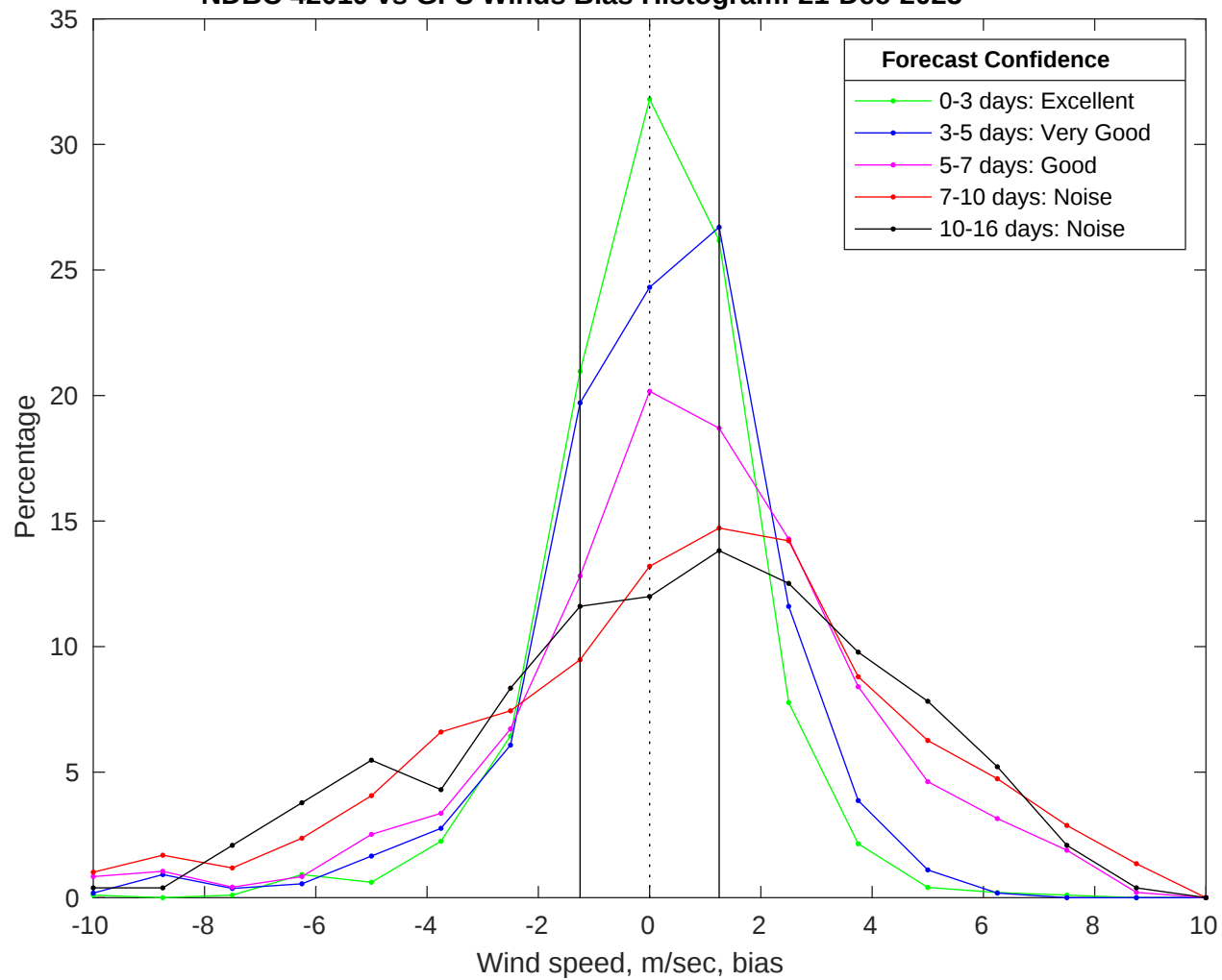
NDBC 42019 vs GFS Winds Bias Histogram: 21-Dec-2025
