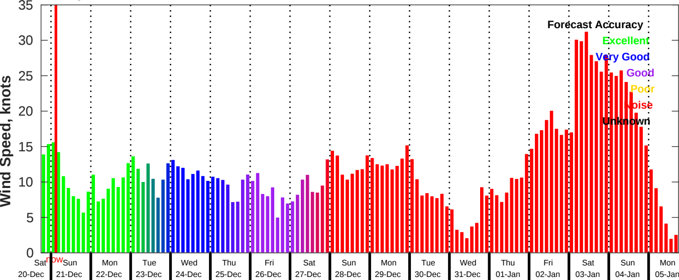
GFS Wind Speed Forecast for NDBC 42019 from 20-Dec-2025 18:00:00 to 05-Jan-2026 18:00:00
