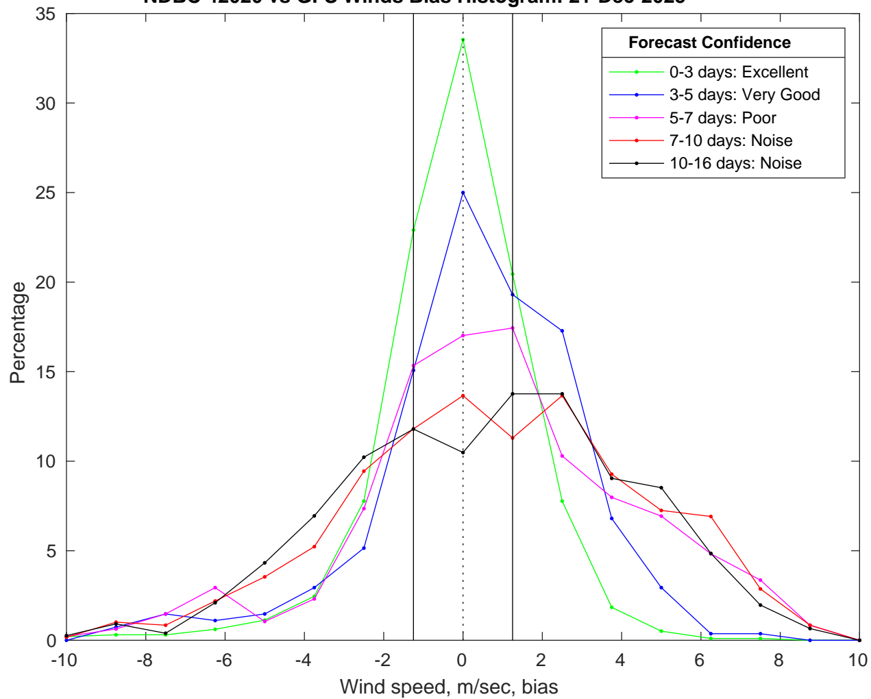
NDBC 42020 vs GFS Winds Bias Histogram: 21-Dec-2025
