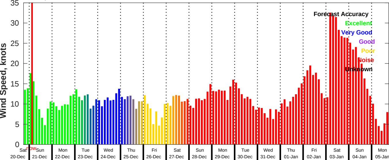
GFS Wind Speed Forecast for NDBC 42020 from 20-Dec-2025 18:00:00 to 05-Jan-2026 18:00:00
