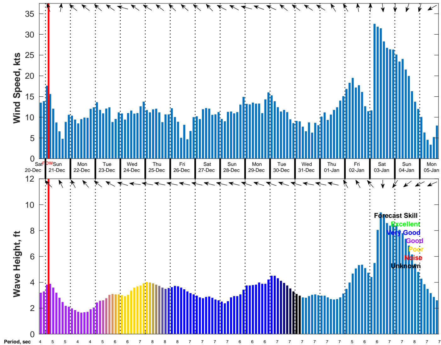
Wind & Wave Forecast for NDBC 42020 from 20-Dec-2025 18:00:00 to 05-Jan-2026 18:00:00
