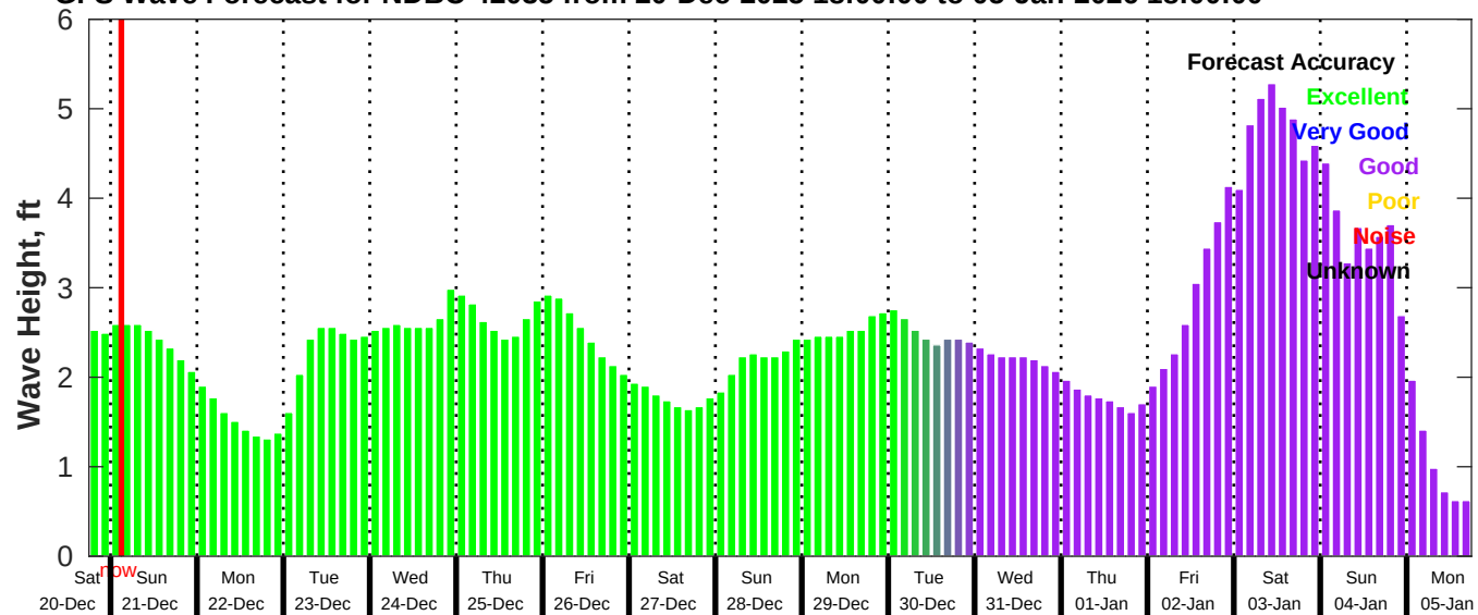
GFS Wave Forecast for NDBC 42035 from 20-Dec-2025 18:00:00 to 05-Jan-2026 18:00:00
