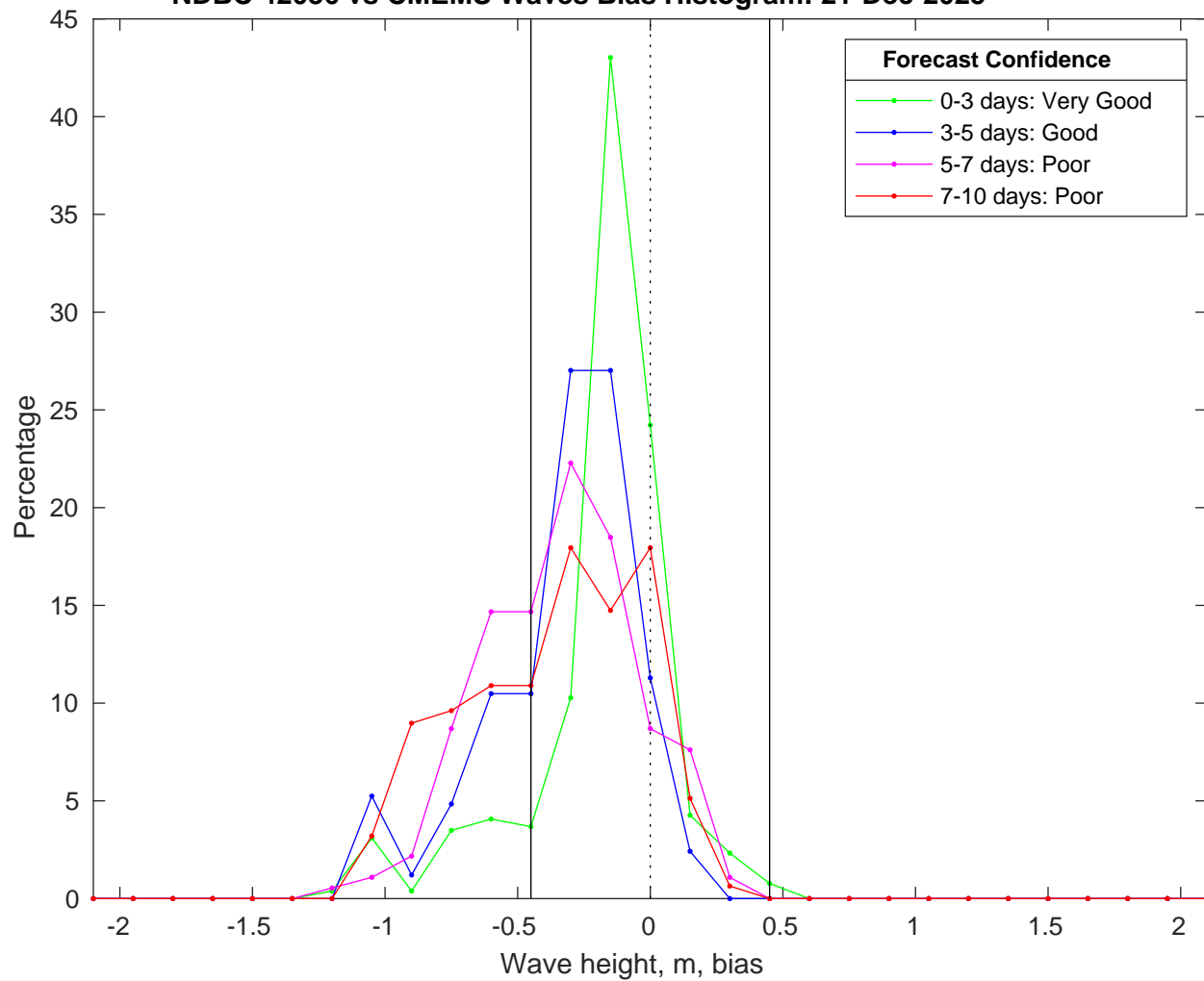
NDBC 42036 vs CMEMS Waves Bias Histogram: 21-Dec-2025
