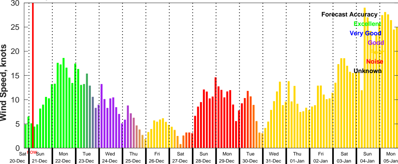
GFS Wind Speed Forecast for NDBC 42036 from 20-Dec-2025 19:00:00 to 05-Jan-2026 19:00:00
