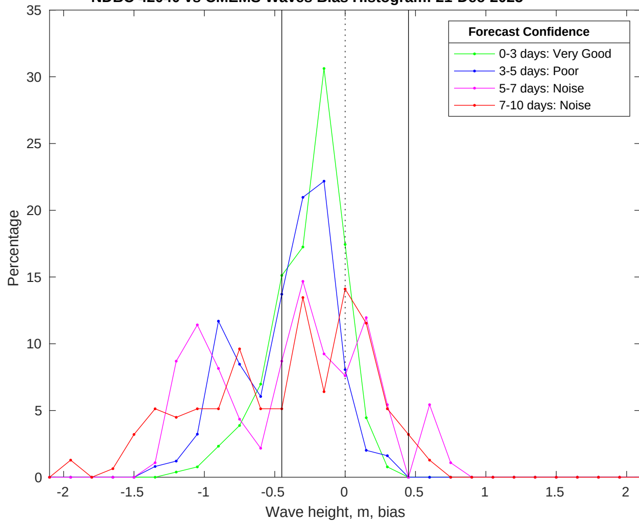
NDBC 42040 vs CMEMS Waves Bias Histogram: 21-Dec-2025
