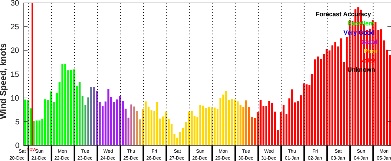
GFS Wind Speed Forecast for NDBC 42040 from 20-Dec-2025 19:00:00 to 05-Jan-2026 19:00:00
