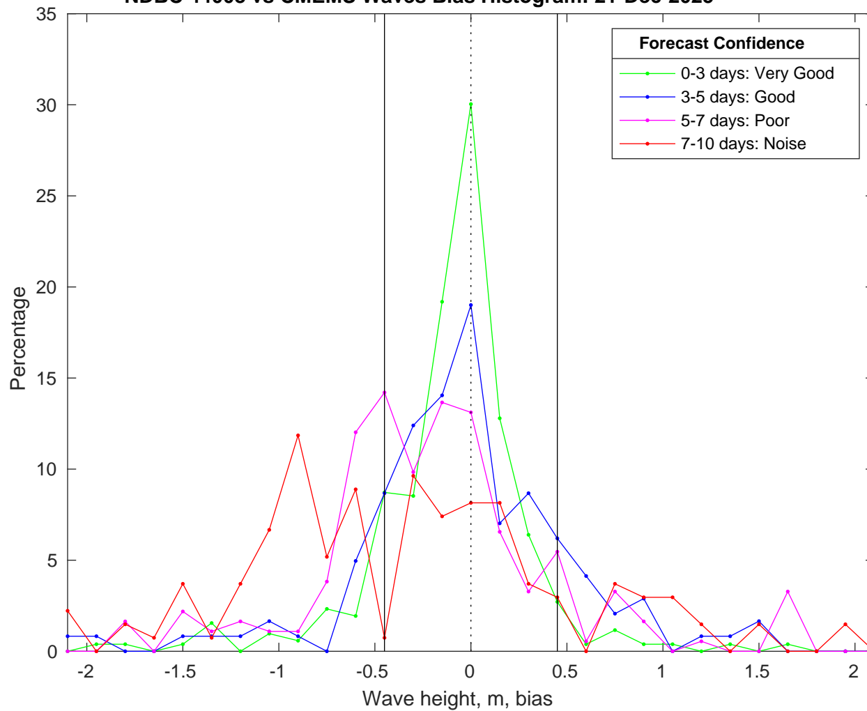
NDBC 44008 vs CMEMS Waves Bias Histogram: 21-Dec-2025
