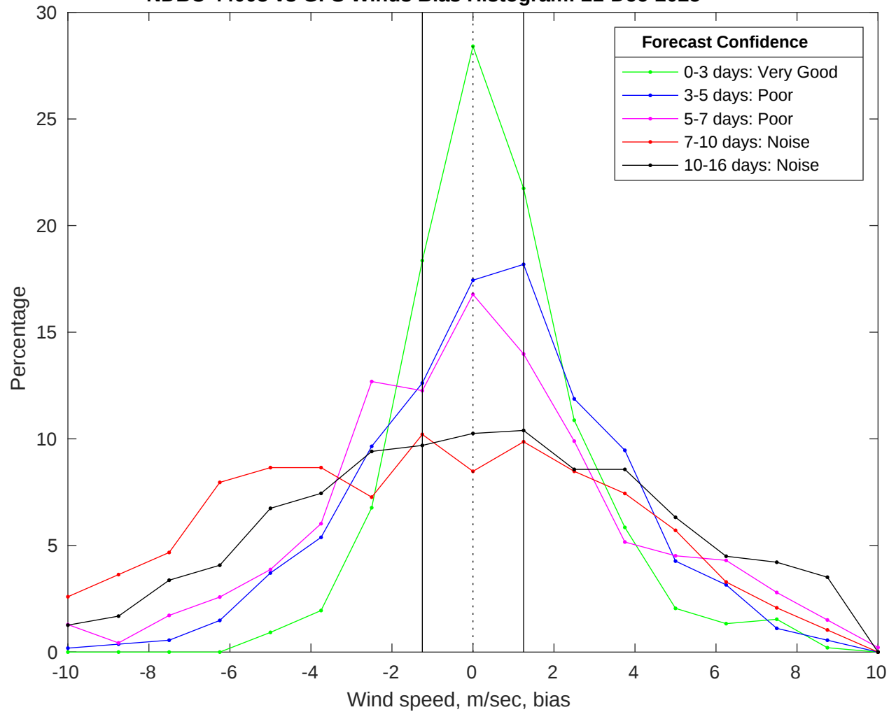
NDBC 44008 vs GFS Winds Bias Histogram: 21-Dec-2025
