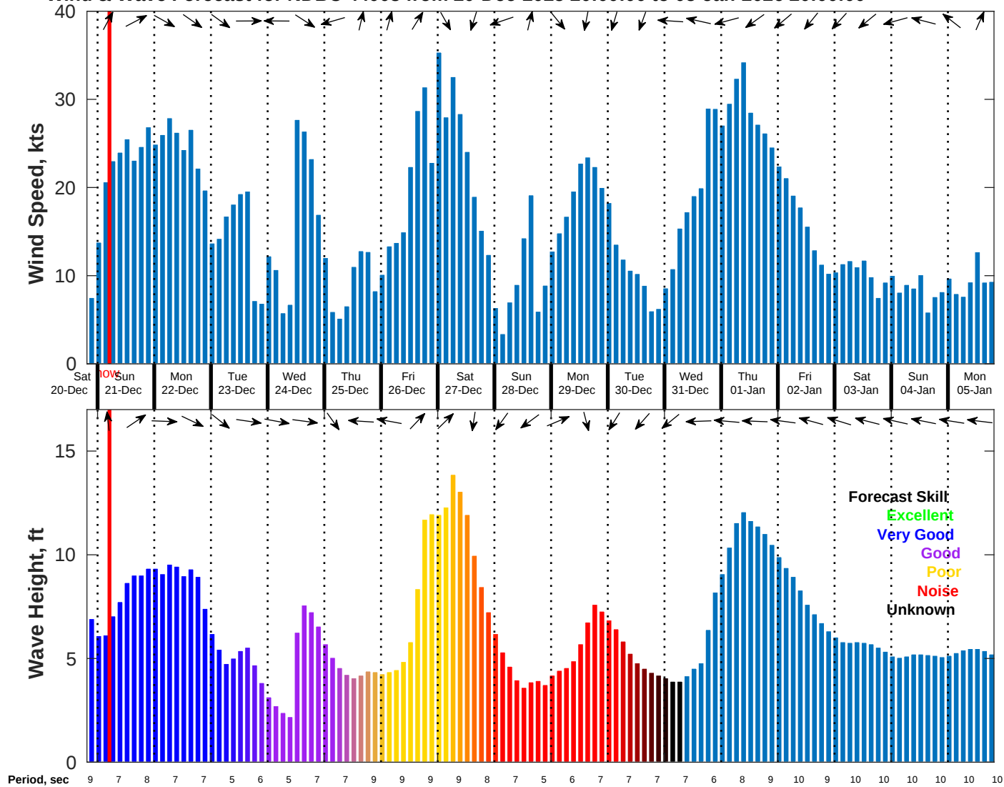
Wind & Wave Forecast for NDBC 44008 from 20-Dec-2025 20:00:00 to 05-Jan-2026 20:00:00
