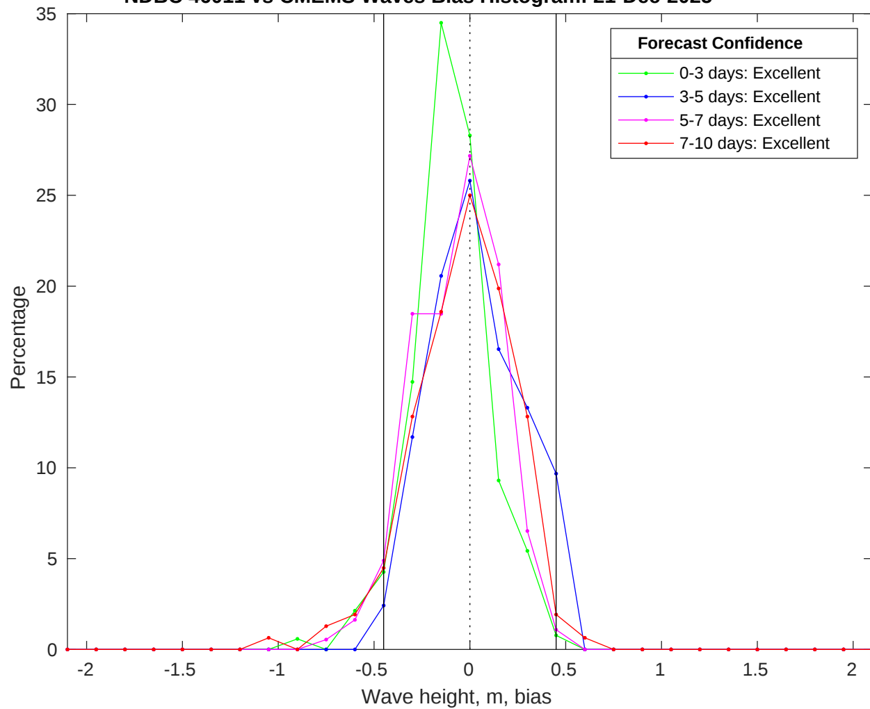
NDBC 46011 vs CMEMS Waves Bias Histogram: 21-Dec-2025
