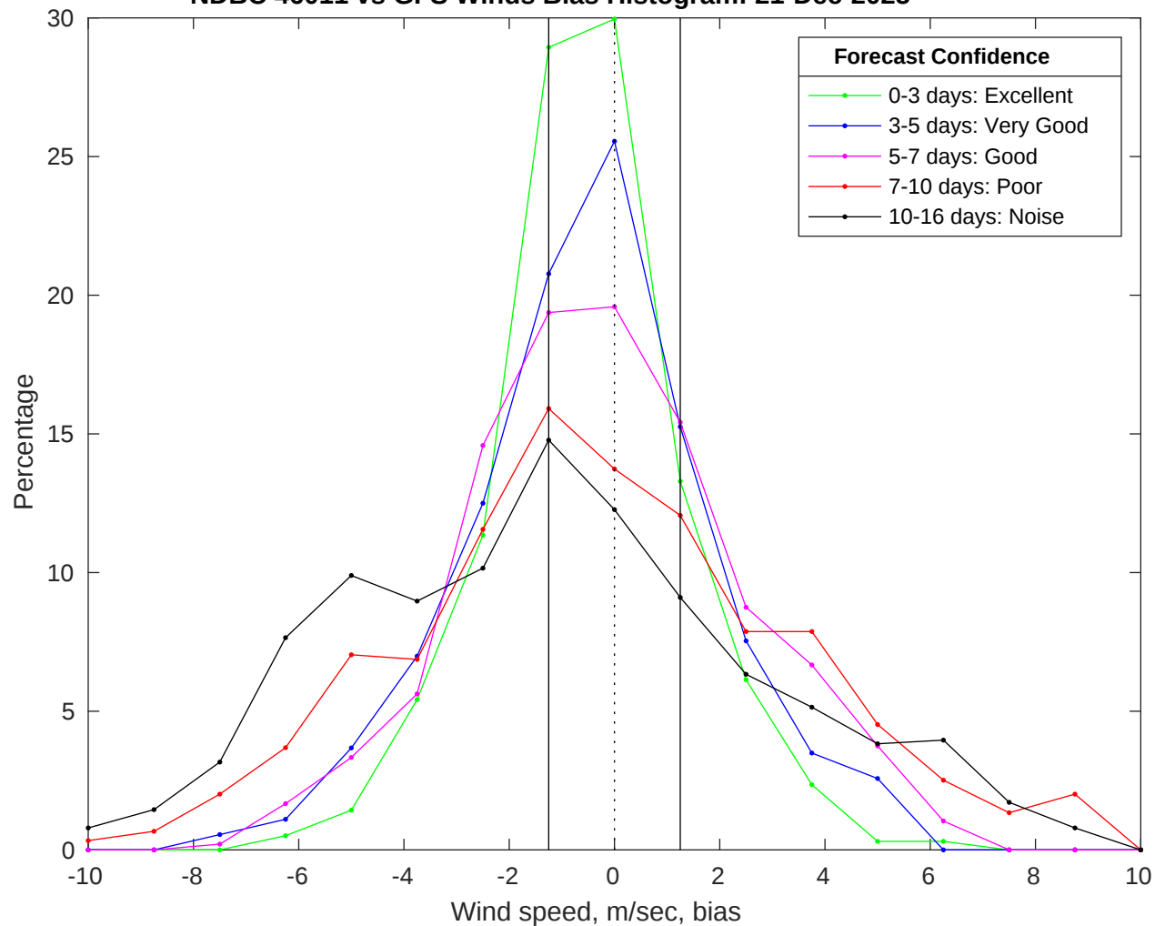
NDBC 46011 vs GFS Winds Bias Histogram: 21-Dec-2025
