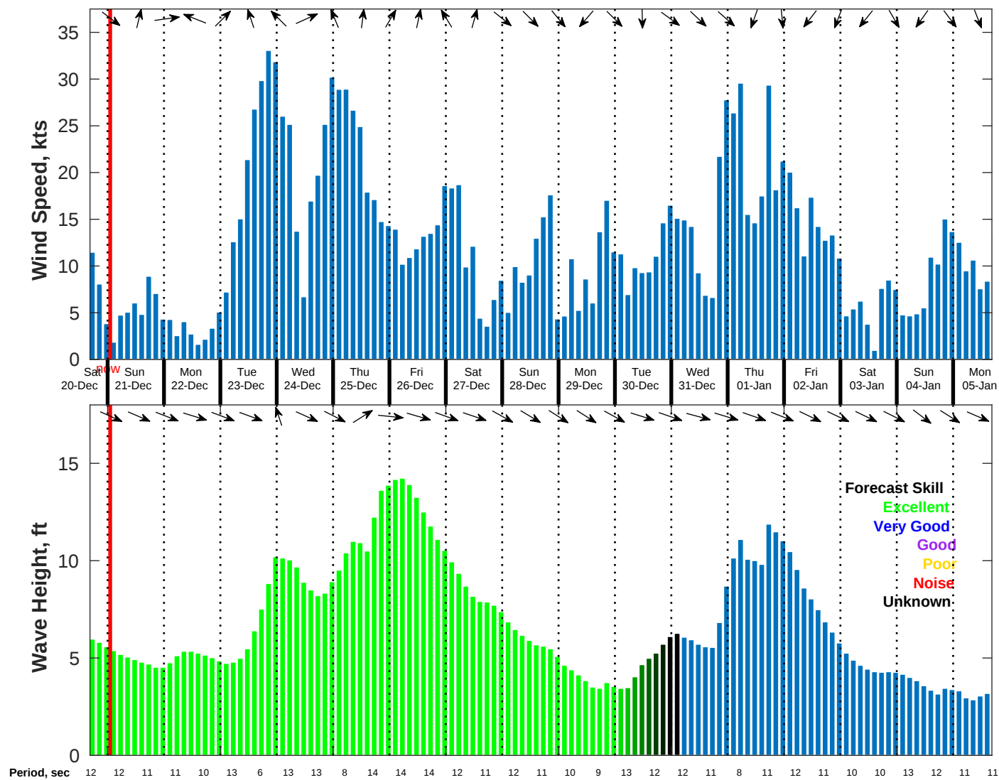
Wind & Wave Forecast for NDBC 46011 from 20-Dec-2025 16:00:00 to 05-Jan-2026 16:00:00
