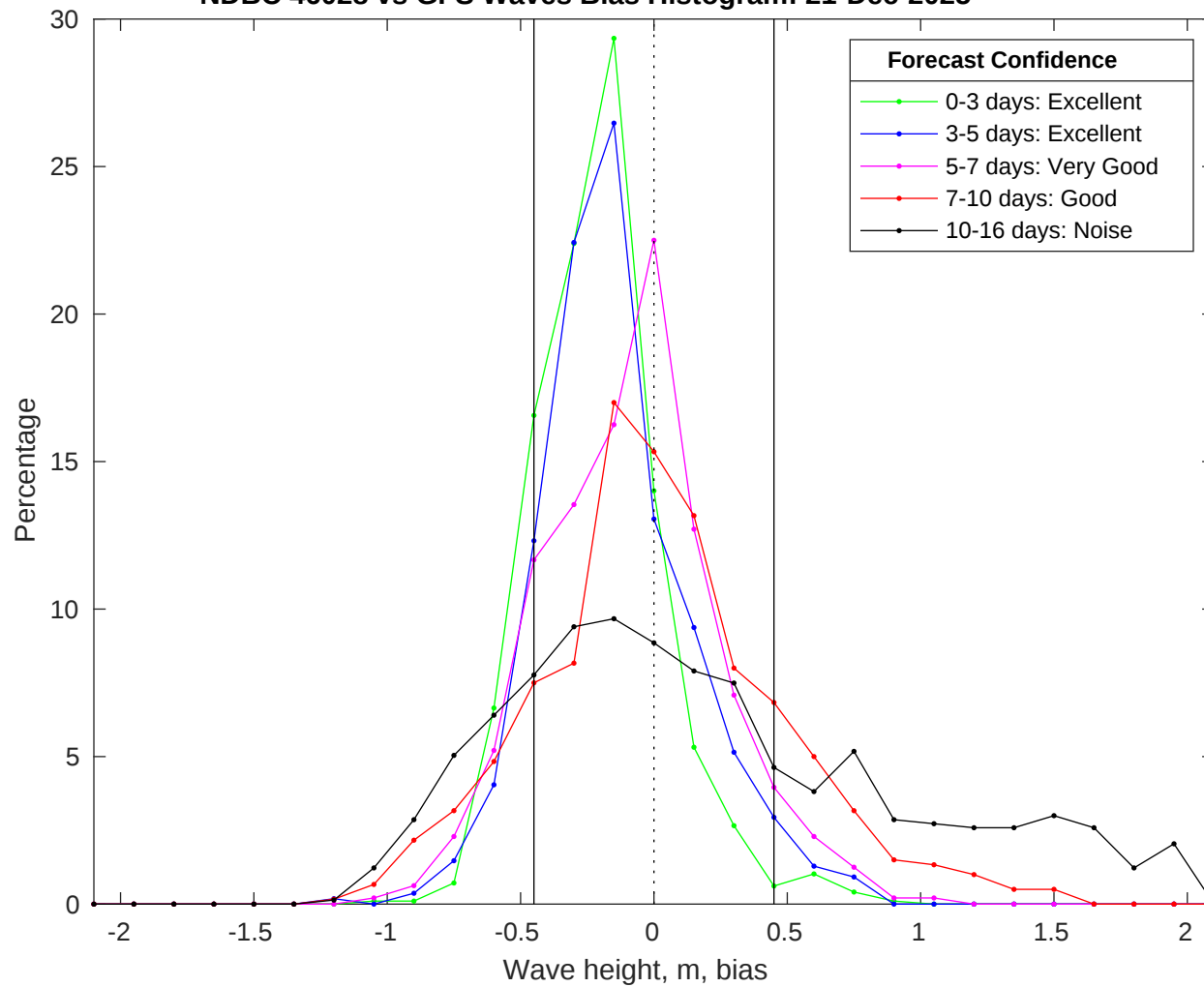
NDBC 46028 vs GFS Waves Bias Histogram: 21-Dec-2025
